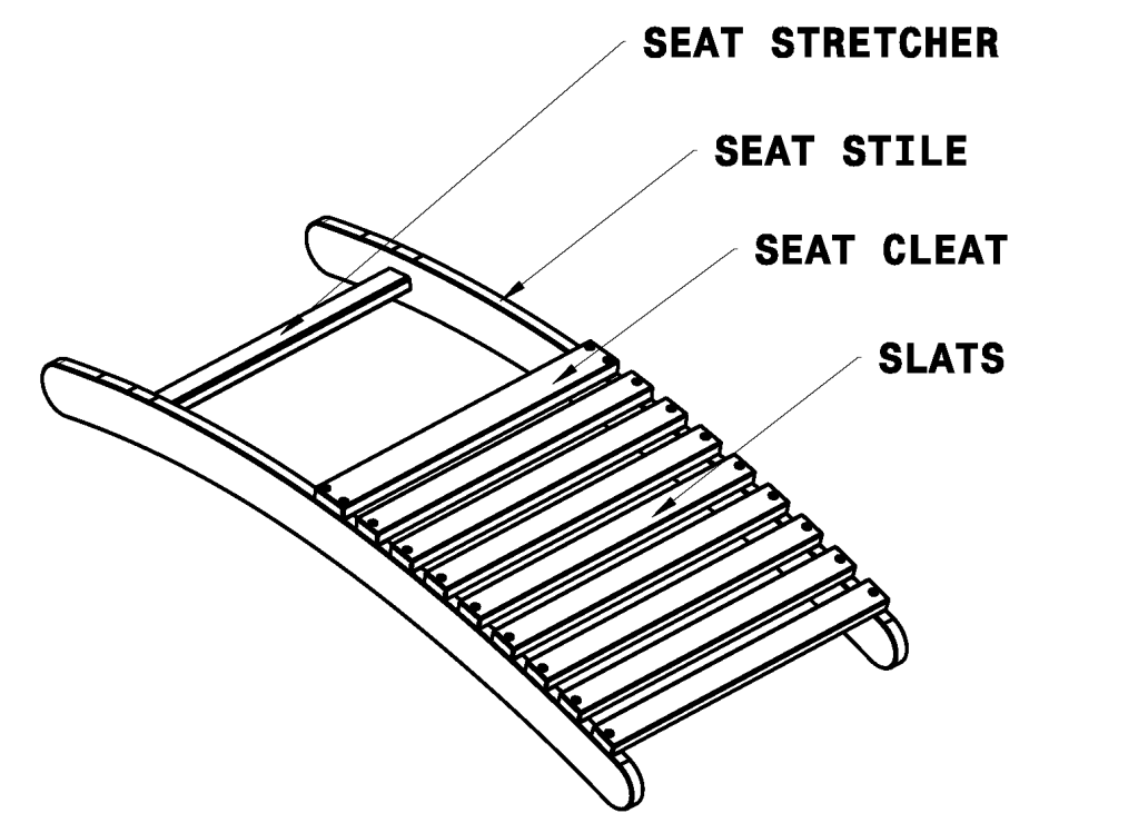
Seat Assy Isometric view Scale: 1:10
