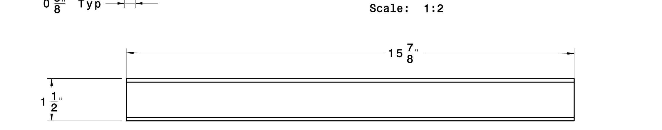
Seat Stretcher view Scale: 1:2
