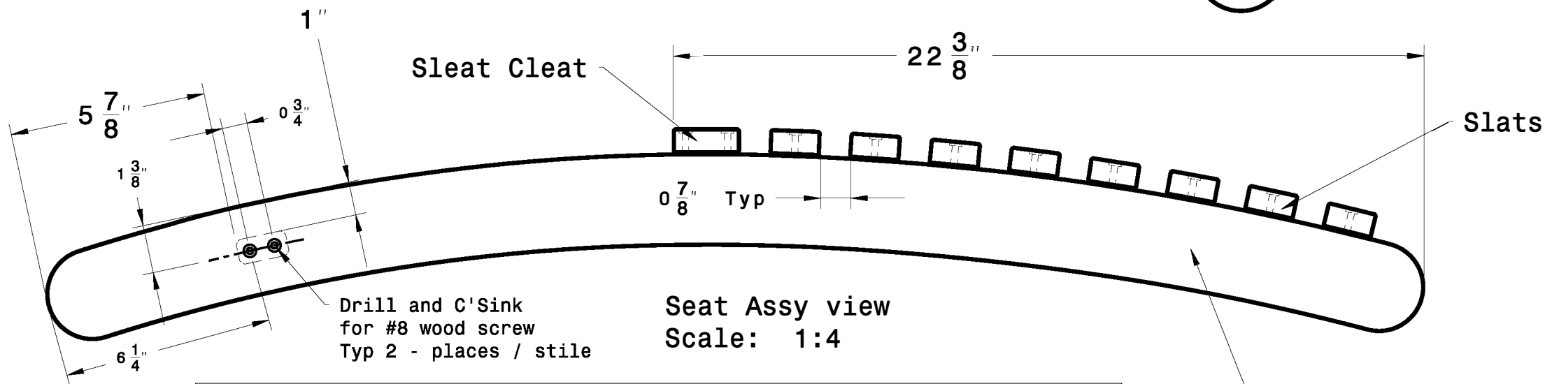
Back Rest Assy view Scale: 1:4
