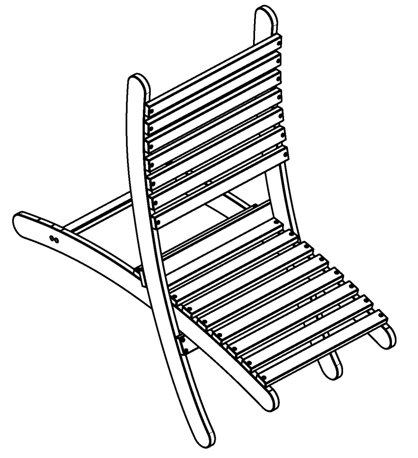
Berg's Camp Chair Isometric view Scale: 1:10
