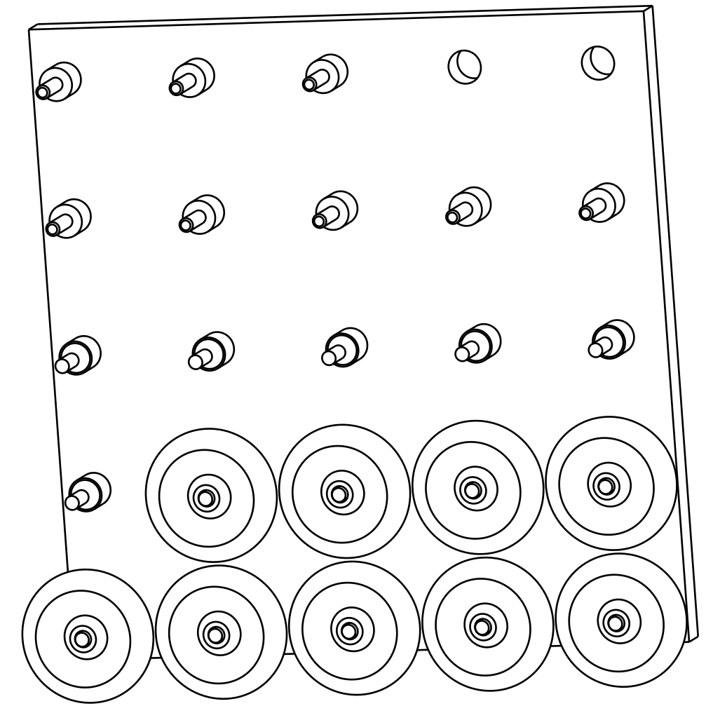
Assembly Isometric view Scale: 1:2
