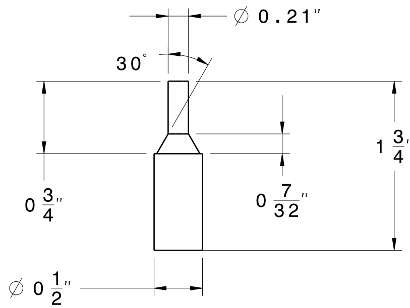
Standoff Front view Scale: 1:1
