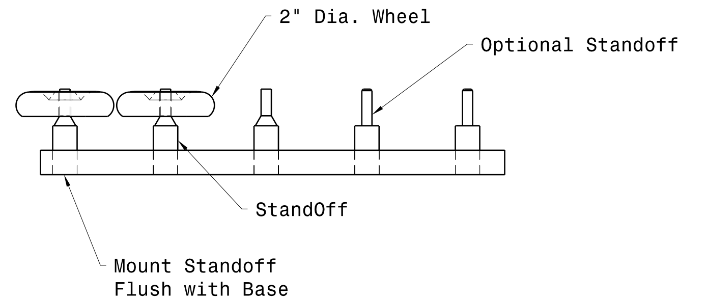
Assembly Front view Scale: 1:2
