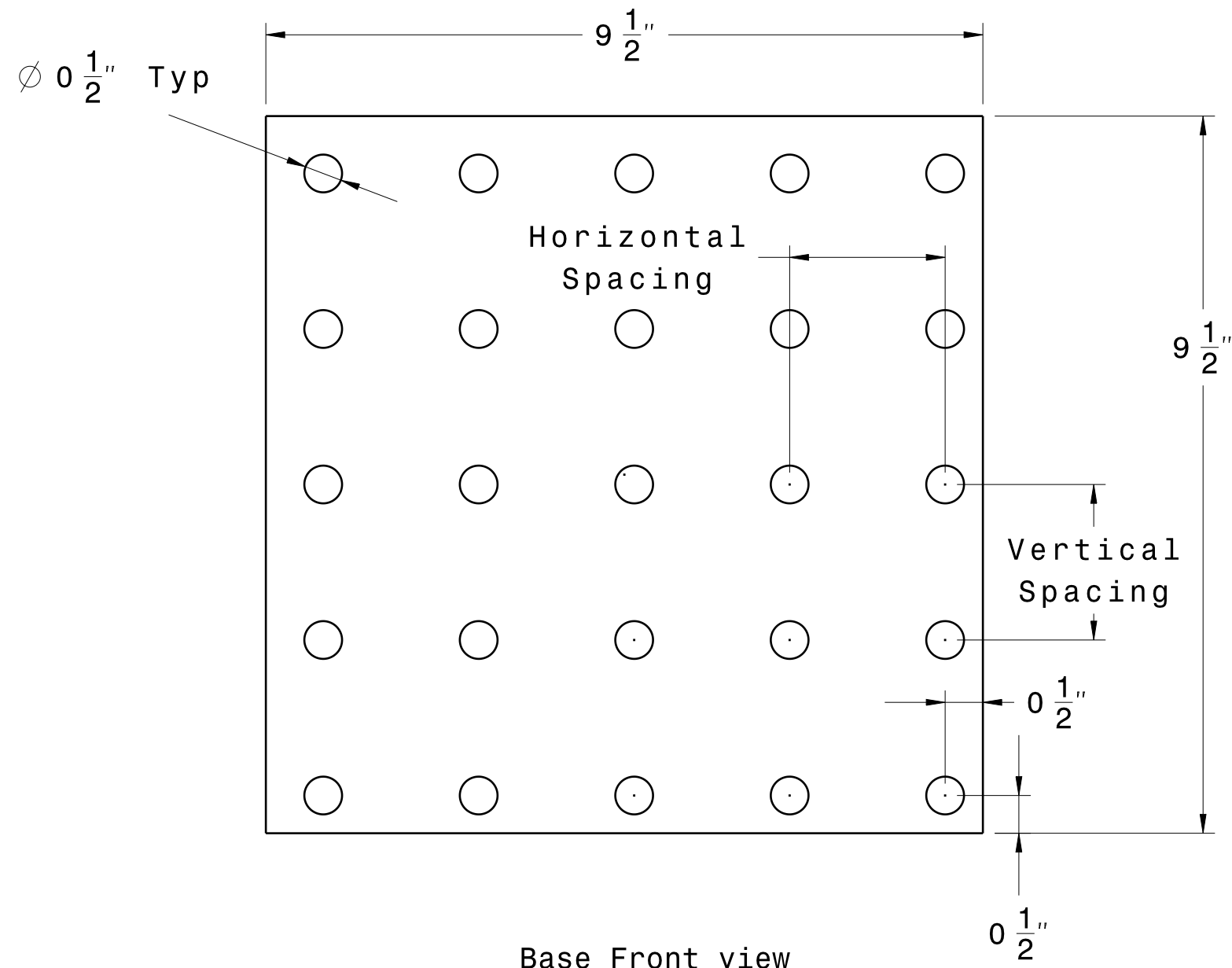
Base Front view Scale: 1:2
