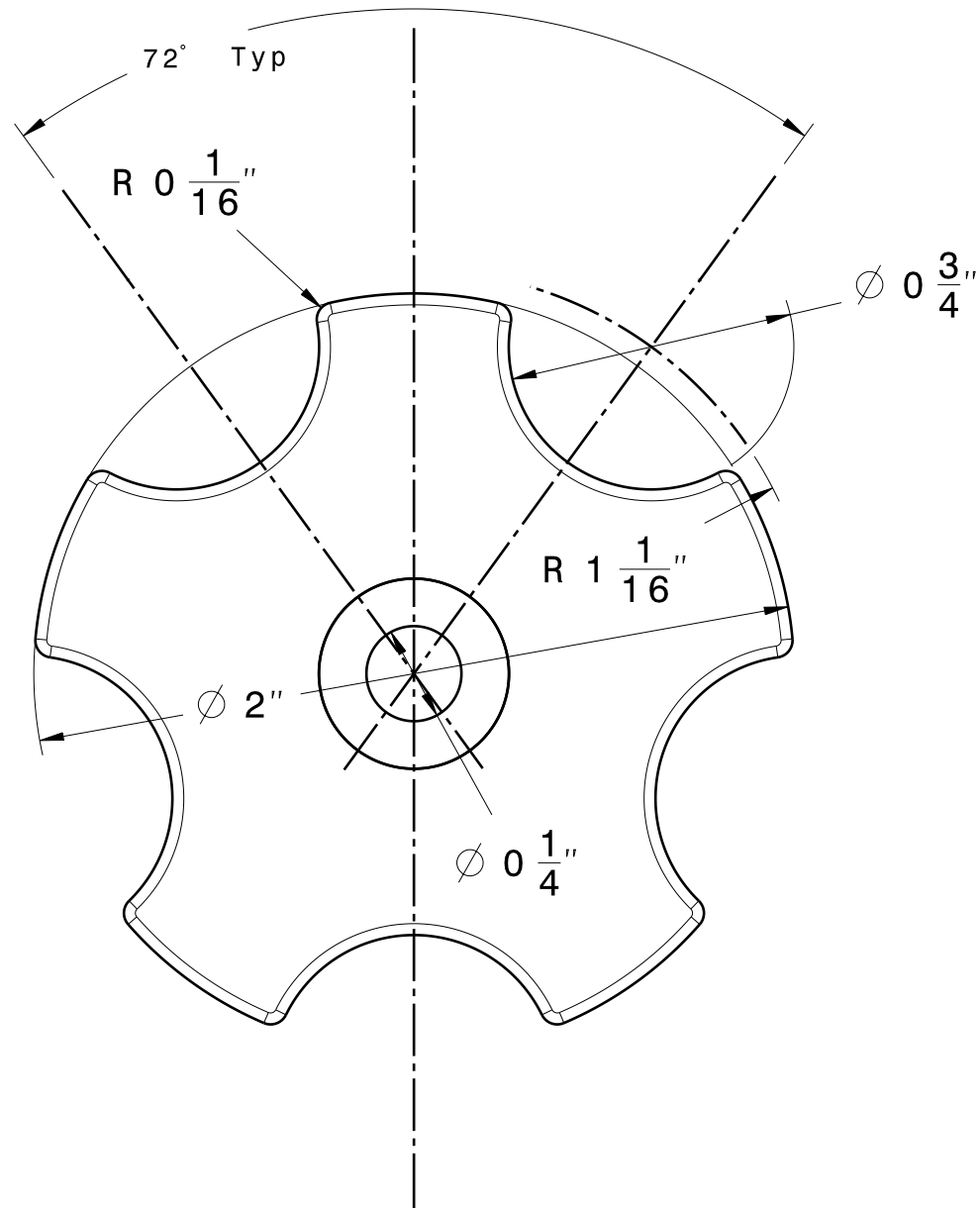
Fluted Knob Front view Scale: 2:1
